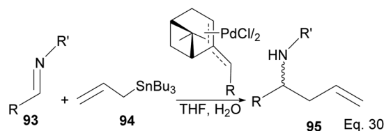
Scheme 26 (–)- \beta -Pinene-based \pi -allylpalladium assisted enantioselective allylation of imine.
