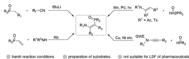
(B) This work: three-component aminophosphylation of maleimides
