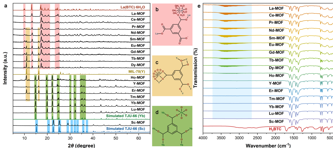
Fig. 4 Comparison of different topologies from RE-MOFs. (a) (from top to bottom) Simulated PXRD patterns of La(BTC)-6H 2 O with CCDC 290771, † experimental PXRD patterns of the prepared RE-MOF (RE = La, Ce, Pr, Nd, Sm, Eu, Gd, Tb or Dy), simulated PXRD pattern of MIL-78 (Y) with CCDC 1109360, † prepared RE-MOF (RE = Ho, Y, Er, Tm, Yb or Lu), simulated PXRD pattern of TJU-66 (Yb), experimental PXRD pattern of prepared Sc-MOF, and simulated PXRD pattern of TJU-66 (Sc); (b–d) Structural formulae for La(BTC)-6H 2 O, MIL-78 (Y) and TJU-66 (Yb); (e) (from top to bottom) FTIR absorption spectra of the prepared RE-MOF (RE = La, Ce, Pr, Nd, Sm, Eu, Gd, Tb, Dy, Ho, Y, Er, Tm, Yb, Lu or Sc), and H 3 BTC, respectively.
