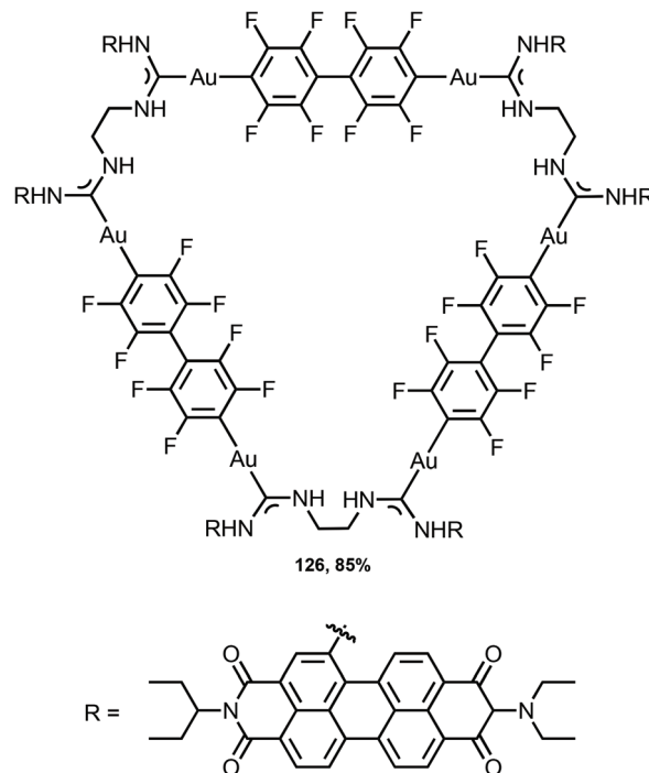
Scheme 19 Preparation of complexes 122–126 . 157
