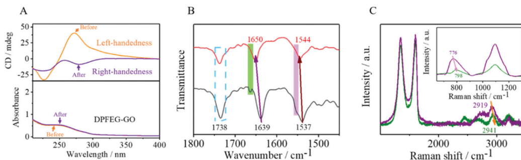
Fig. 2 CD and corresponding UV-vis spectra of (A) DPFEF-GO 3% before and after IR irradiation. (B) FTIR and (C) Raman of DPFEF-GO 3% hydrogels.
