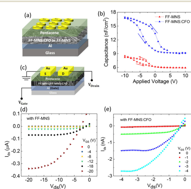
Fig. 5 FF-MNS nanocomposites in transistors. (a) Schematic of a pentacene MIS diode. (b) Capacitance–voltage characteristics of pentacene MIS diodes using as-is FF-MNS and CFO functionalized FF-MNS dielectric layers. (c) Schematic of an FET. (d) and (e) Output characteristics of pentacene FETs with as-is FF-MNS and CFO functionalized FF-MNS dielectrics, respectively. Reprinted with permission from ref. 22, copyright 2018, American Chemical Society.
