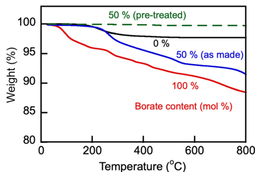
Fig. 2 TGA heating ramp ( 10 \text{ }^\circ\text{C min}^{-1} ) of as-made carbonate ( \text{Li}_{1.24}\text{K}_{0.76}\text{CO}_3 ), borate ( \text{Li}_{1.5}\text{Na}_{1.5}\text{BO}_3 ) and as-made and pre-treated blend (1:1 mol/mol, sample no. 3 in Table 1) in nitrogen atmosphere. The blend sample was pre-treated by its equilibration at 600 \text{ }^\circ\text{C} in \text{N}_2 atmosphere for 1 h. Numbers stand for nominal initial content of borate (mol%) in the samples.
