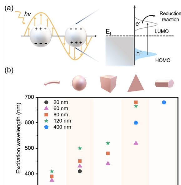
Fig. 2 (a) The mechanism of the LSPR effect within Ag nanoparticles. (b) Plasmon excitation peaks of different Ag morphologies and sizes, the “size” represents the diameter of sections (nanowire/penta-twinned crystalline nanowires, nanosphere and nanoprism), diameter and length of sides of nanocubes, respectively.
