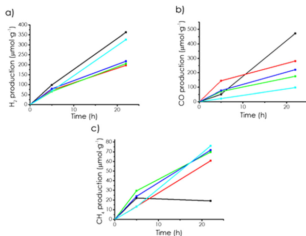
Fig. 4 Temporal profiles of (a) H 2 , (b) CO, and (c) CH 4 evolution for mp-C α (black), mp-C β (red), mp-C γ (green), mp-(N)-C α (blue), and mp-(P)-C α (cyan) upon the irradiation of CO 2 dissolved in CH 3 CN/H 2 O containing TEOA with the output of a 300 W Xe lamp.
