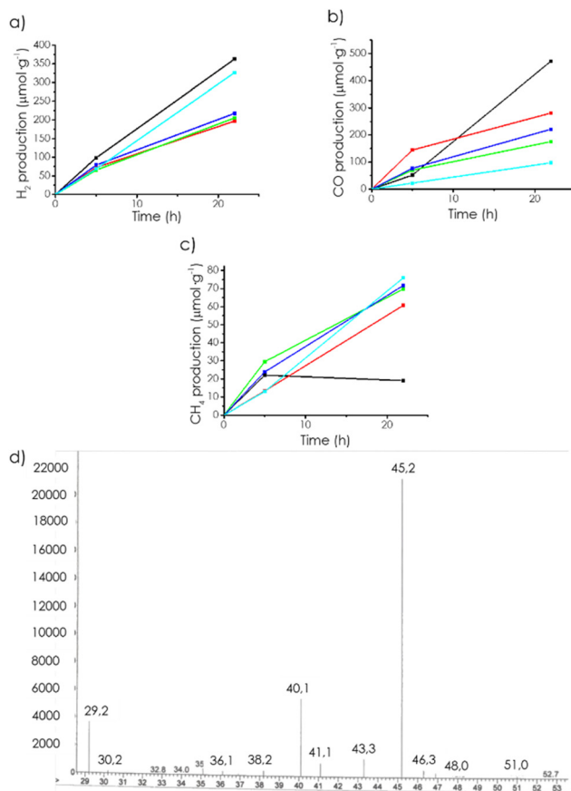
Fig. 3 Temporal gas evolution from CO 2 dissolved in a CH 3 CN/H 2 O mixture containing TEOA using mp-C α (black), mp-C β (red), mp-C γ (green), mp-(N)-C α (blue), and mp-(P)-C α (cyan) as photocatalysts upon 300 W Xe lamp irradiation: (a) H 2 , (b) CO, (c) CH 4 , (d) mass spectra of the test using 13 CO 2 as the substrate and mp-C α as the photocatalyst.
