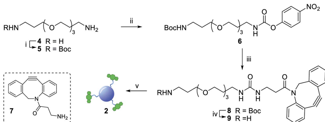
Scheme 1 Reagents and conditions: (i) Boc 2 O, DCM, 4 h, 0 °C to rt, 99%; (ii) 4-nitrophenyl chloroformate, Py, DCM, 3 h, 0 °C to rt, 87%; (iii) 7, Py, DIPEA, DMF, 63%; (iv) TFA, DCM, 1.5 h, rt, 86%; (v) 3, HATU, DIPEA, DMF, 5 h, rt.
