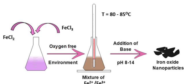
Fig. 3 Steps to synthesize IONPs through the co-precipitation method. Fe 2+ and Fe 3+ are added in a 2:1 molar ratio in an oxygen-free environment and heated to 80–85 °C followed by the addition of base. The precipitated particles are then centrifuged or magnetically separated.
