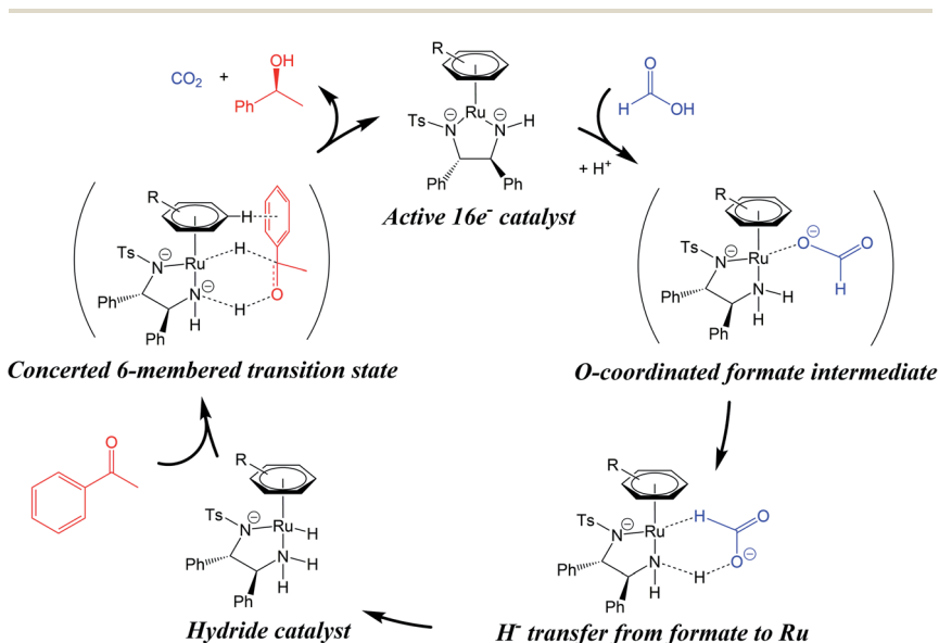
Fig. 1 The classical TH mechanism for ruthenium arene catalysts. The hydride catalyst is generated from a hydride source (formic acid, blue) which may involve carboxylate O -coordination to the metal centre. Reduction of the prochiral substrate (acetophenone, red) is thought to involve a 6-membered concerted transition state. A CH/ \pi interaction is shown between the \eta^6 -arene of the catalyst hydride complex, and the arene substituent of the substrate. Based on ref. 10.
