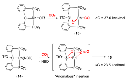
Scheme 3 DFT calculated pathways for CO 2 reductive cleavage of CO 2 into CO and siloxide by complex 14 . Top: silylene pathway, bottom: anomalous insertion pathway.
