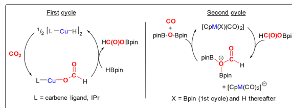
Scheme 43 Mechanism for the 2-electron reduction of CO 2 to CO catalysed by heterobimetallic complexes [(NHC)Cu–ML n ] {ML n = [FeCp(CO) 2 ], [WCp(CO) 3 ], [MoCp(CO) 3 ]}. X = Bpin (1st cycle) and H thereafter
