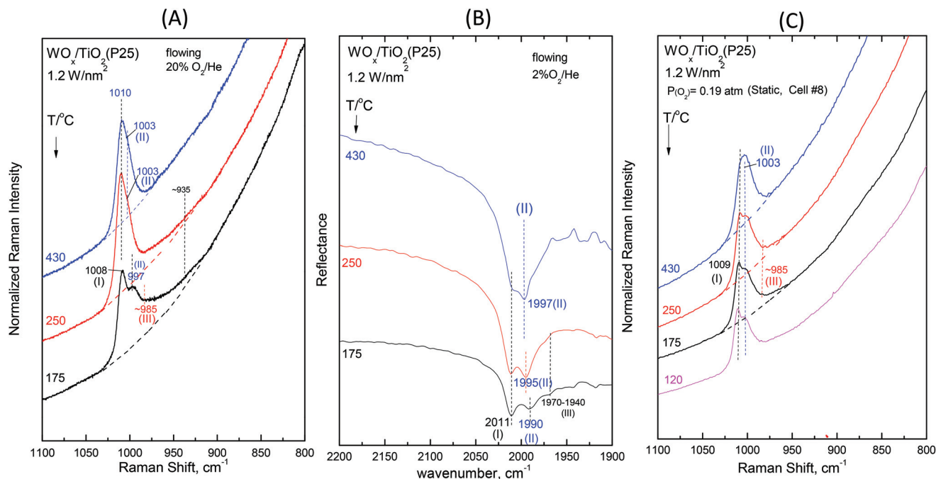
Fig. 2 \text{WO}_x/\text{TiO}_2(\text{P25}) with a surface density of 1.2 \text{ W nm}^{-2} : (A) Sequential in situ Raman spectra obtained under flowing 20\% \text{ O}_2/\text{He} at temperatures as indicated by each spectrum. Recording parameters: laser wavelength, \lambda_0 = 491.3 \text{ nm} ; laser power, w = 10 \text{ mW} ; time constant, \tau = 1.2 \text{ s} ; and spectral slit width, \text{ssw} = 8 \text{ cm}^{-1} . (B) Sequential in situ FTIR spectra obtained under flowing 2\% \text{ O}_2/\text{He} at temperatures as indicated by each spectrum. (C) Sequential Raman spectra at static equilibrium under p_{\text{O}_2} = 0.19 \text{ atm} at temperatures as indicated by each spectrum; spectral parameters: \lambda_0 = 532.0 \text{ nm} ; laser power, w = 20 \text{ mW} ; resolution, 2 \text{ cm}^{-1} .
