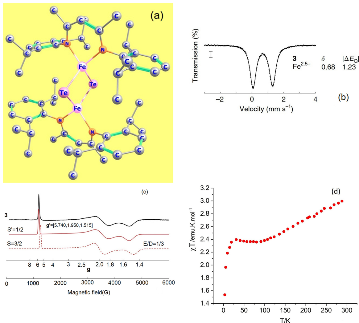
Fig. 2 Experimental X-ray structure of the mixed valence complex \text{Fe}^{2.5+}_{-\mu}\text{Te}_2\text{Fe}^{2.5+} (a); its T = 80 K Mössbauer spectrum in zero magnetic field (b); continuous-wave X-band EPR spectrum (9.63 GHz) of a frozen solution at 3.6–8 K, collected under non-saturating microwave power conditions (black line) and simulations (red lines): pseudo-spin S' = 1/2 , g' = 5.740, 1.950, 1.515 (solid red line) and a S = 3/2 , spin-Hamiltonian, |D| \gg h\nu , |E/D| = 1/3 (assuming g = g_e = 2.0023 ) and a value of D < 15 \text{ cm}^{-1} , estimated from the temperature dependence of the Lorentzian linewidth (c), variable-temperature SQUID magnetic susceptibility of a solid sample (d); data have been reproduced in a modified form from J. T. Henthorn, G. E. Cutsail III, T. Weyhermüller and S. DeBeer, "Stabilization of intermediate spin-states in mixed-valence diiron dichalcogenide complexes", Nat. Chem. , https://doi.org/10.1038/s41557-021-00853-5 .
