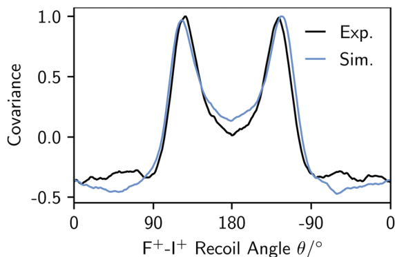
Fig. 3 Experimental (black) and simulated (blue) F^+ - I^+ angular distributions from the analogous \text{Cov}(F^+, I^+) images in Fig. 2.
