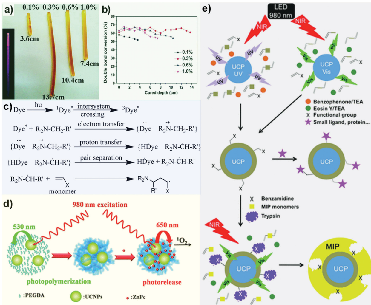
Fig. 4 (a) Curing depths obtained using different concentrations of NaF 4 :Yb 3+ , Tm 3+ UCNC. 81 (b) Degree of monomer conversion at different curing depth. 81 Reprinted with permission from ref. 81. Copyright 2016, Royal Society of Chemistry. (c) Key steps to generate free radicals by the dye/coinitiator system. 82 Reprinted with permission from ref. 82. Copyright 2008, Wiley-VCH. (d) Schematic illustration of NIR light-activated photopolymerization of PEGDA hydrogels and NIR light-controlled release of singlet oxygen from ZnPc loaded into UCNP-PEGDA hybrid microspheres. 83 Reprinted with permission from ref. 83. Copyright 2013, Royal Society of Chemistry. (e) Schematic illustration of a generalized strategy to coat a polymer shell with different functional groups (X) on UCNC via UCNC-assisted photopolymerization and to further coat a molecularly imprinted polymer (MIP) layer in the presence of a molecular template (e.g., trypsin) and MIP monomers. 84 Reprinted with permission from ref. 84. Copyright 2014, Wiley-VCH.
