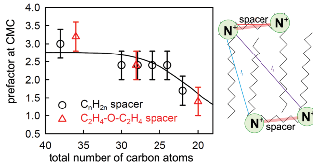
Fig. 8 The experimentally determined prefactor P in the Gibbs equation at the CMC (points) of C_n\text{NMe}_2\text{C}_6\text{NMe}_2\text{C}_n\text{Br}_2 (black circles) and C_n\text{NMe}_2\text{C}_2\text{-O-C}_2\text{NMe}_2\text{C}_n\text{Br}_2 (red triangles) and a calculated value (line) based on the structure shown alongside and a model described in the text. The two points at 28 carbons have been laterally displaced from each other for clarity. Key distances between charged groups are marked in the structure shown. Figure redrawn from Li et al. 80
