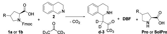
Scheme 3 Reaction conditions for the cross-catalytic reaction used in this study. 1a or 1b (133 mM) is reacted with 2 (133 mM) in acetone- d_6 at 25 °C for 12 hours.
