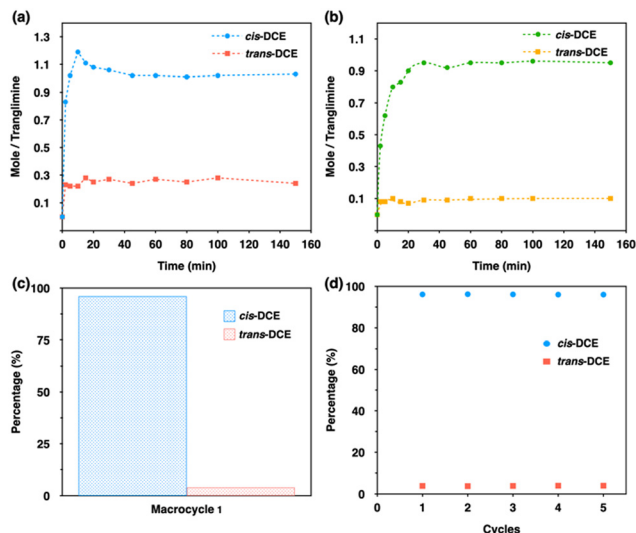
Fig. 4 (a) Time-dependent solid–vapor sorption plot of 1a for single-component cis - and trans -DCE. (b) Time-dependent solid–vapor sorption plot of 1a in cis/trans -DCE (1:1 v/v) mixture. (c) Relative uptake of cis - and trans -DCE over 1 h. (d) Relative uptake capacity of crystalline 1A towards cis/trans -DCE (1:1 v/v) mixture for 5 cycles.
