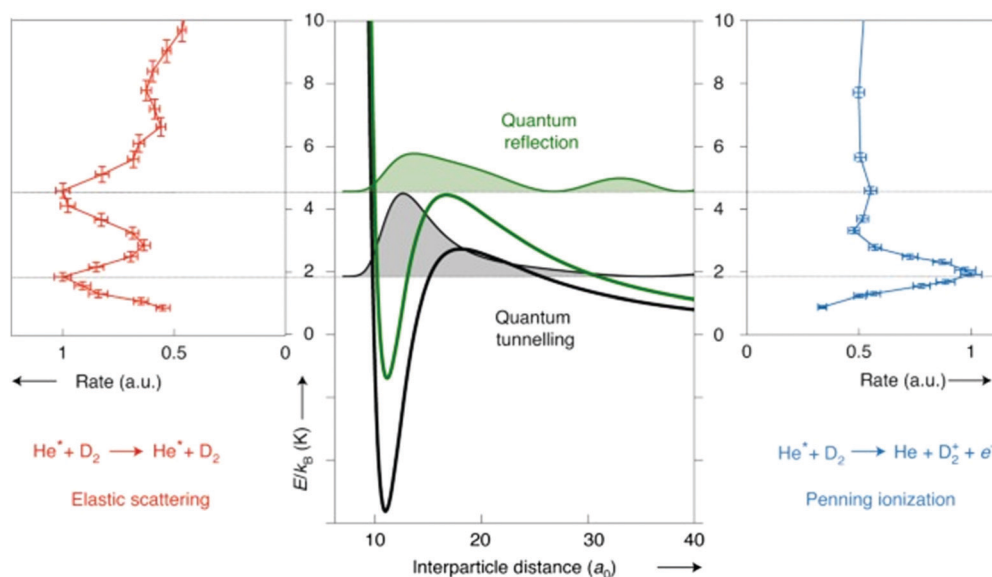
Fig. 1 Schematic illustration of the different types of resonances present in the Penning ionisation and elastic scattering pathways following collisions between metastable He and \text{D}_2 . Note that metastable He, denoted \text{He}^* in the figure, is a triplet radical species. At collision energies that coincide with the location of partial waves (with the squared resonance wavefunctions shown shaded in black and green on the central panel), peaks are seen in the rate coefficient plots. Adapted from Paliwal et al. , copyright 2021, under exclusive licence to Springer Nature Limited. 13
