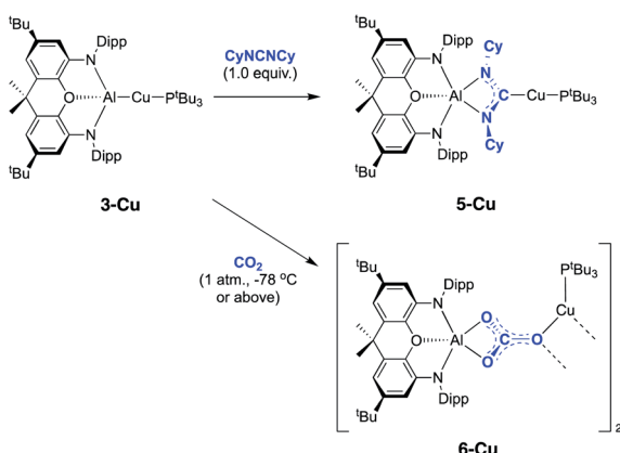
Scheme 4 Reactions of copper-aluminum compound 3-Cu with \text{CO}_2 and CyNCNCy.
