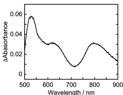
Fig. 7 Difference absorption spectrum from before and after electrocyclic one-electron reduction of Os. A CO 2 -saturated DMA solution containing Os (0.5 mM) and Et 4 NBF 4 (0.1 M) as an electrolyte was reduced at -1.75 V using a UV-vis OTTLE cell with a Pt mesh working electrode and Ag/AgNO 3 reference electrode.
