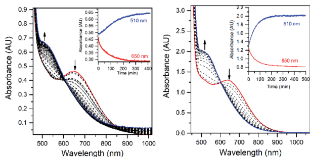
Fig. 8 Electronic absorption spectra showing the decay of anaerobic CH 3 CN solutions of 2 mM [Mn III (OO t Bu)( 6 Me 6 dpaq)] + and 6 mM [Mn III (OOCm)( 6 Me 6 dpaq)] + (red traces) at 323 K to give [Mn III (OH)( 6 Me 6 dpaq)] + (blue traces). The inset shows the change in absorbance at 650 and 510 nm over the course of the decay reaction.
