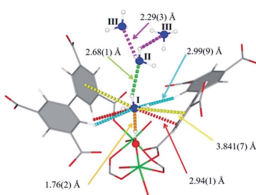
Fig. 19 Binding sites for ND 3 molecules adsorbed within MFM-300(Al) determined by in situ NPD studies. Reprinted with permission from ref. 110. Copyright (2018) John Wiley & Sons.
