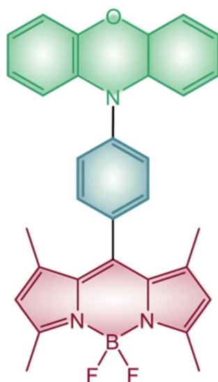
BDP-Ph-PXZ
