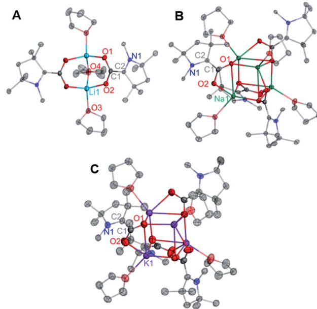
Fig. 2 Solid state molecular structures of 2 (A), 3 (B), and 4 (C). All H atoms and carbon atoms not directly attached to the CAAC core ring are omitted for clarity. Selected bond distances (Å) and angles (degree): 2: O1-C1: 1.2732(12); O2-C1: 1.2778(12); C1-C2: 1.4533(13); N1-C2: 1.3802(12); O1-C1-O2: 123.71(9); O1-C1-C2: 119.84(9); O2-C1-C2: 116.45(9); N1-C2-C1: 124.85(9); N1-C2-C3: 110.81(8). 3: O1-C1: 1.286(3); O2-C1: 1.266(3); C1-C2: 1.458(3); N1-C2: 1.385(3); O2-C1-O1: 122.9(2); O2-C1-C2: 118.7(2); O1-C1-C2: 118.3(2); N1-C2-C1: 124.7(2); N1-C2-C3: 109.7(2). 4: O1-C1: 1.276(6); O2-C1: 1.265(7); C1-C2: 1.451(7); N1-C2: 1.384(6); O2-C1-O1: 123.0(5); O2-C1-C2: 119.1(5); O1-C1-C2: 117.9(5); N1-C2-C1: 123.3(5); N1-C2-C3: 110.2(4).
