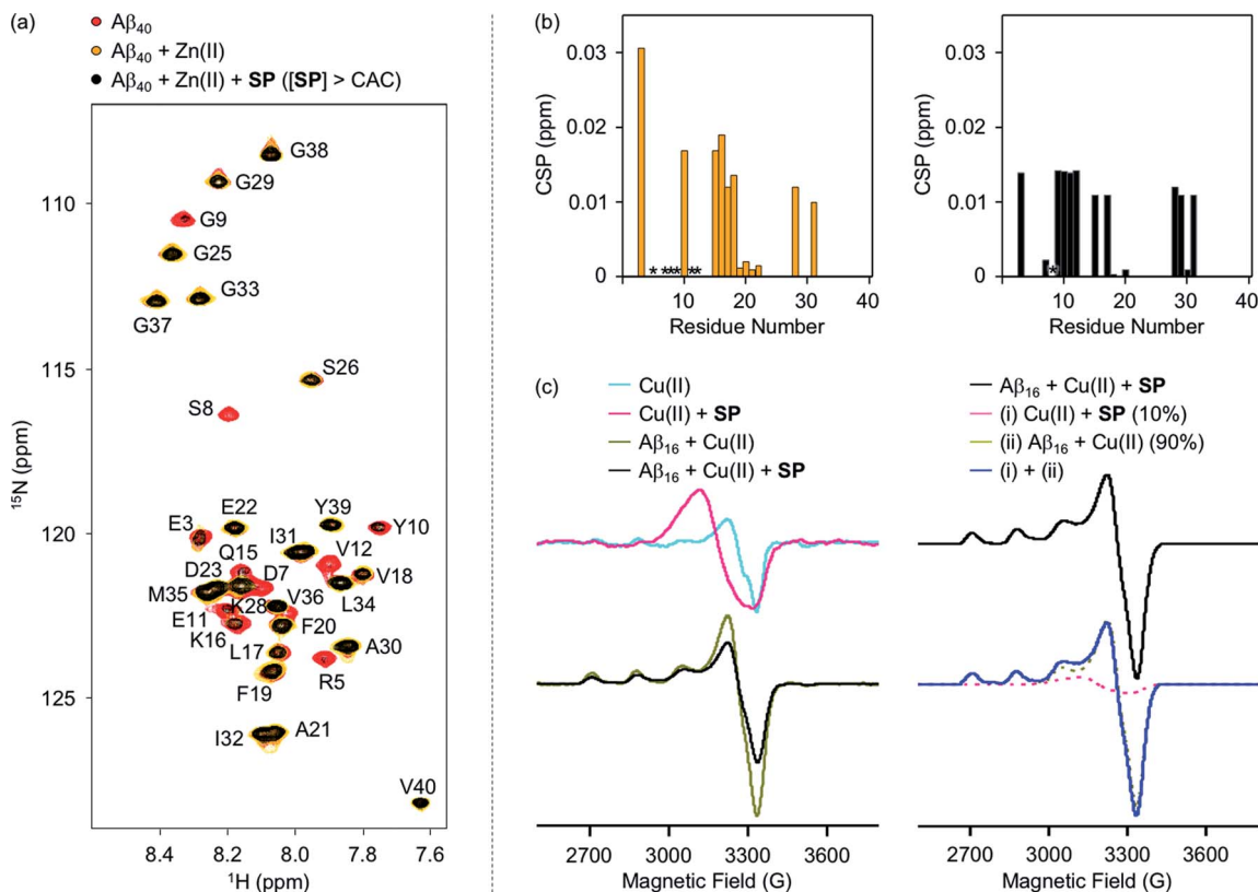
Fig. 5 Interactions of SP with metal–A \beta analyzed by 2D ^1\text{H} – ^{15}\text{N} SOFAST-HMQC NMR and EPR spectroscopy. (a) 2D NMR spectra of ^{15}\text{N} -labeled A \beta_{40} with and without Zn(II) and SP at the concentration above the CAC. (b) CSPs of the Zn(II) samples in the absence (left) and presence (right) of SP at the concentration above the CAC. Upon addition of Zn(II) to the solution of ^{15}\text{N} -labeled A \beta_{40} with and without SP, the NMR signals of the amino acid residues indicated in asterisks (*) disappeared. Conditions: [ ^{15}\text{N} -labeled A \beta_{40} ] = 40 \mu\text{M} ; [Zn(II)] = 40 \mu\text{M} ; [SP] = 100 \mu\text{M} (above the CAC) (1% v/v DMSO); 20 mM HEPES, pH 7.4; 10% v/v D _2 O; 10 ^\circ\text{C} . (c) EPR spectra of the Cu(II) samples with and without SP and A \beta_{16} . The simulated spectrum (blue), similar to the normalized experimental spectrum of the Cu(II) sample with A \beta_{16} and SP (black), was obtained by weighted summation of the normalized spectra of the Cu(II) samples with either SP (10%; pink) or A \beta_{16} (90%; dark yellow). Conditions: [A \beta_{16} ] = 100 \mu\text{M} ; [Cu(II)] = 100 \mu\text{M} ; [SP] = 400 \mu\text{M} (above the CAC) (1% v/v DMSO); 20 mM HEPES, pH 6.8, 150 mM NaCl; 37 ^\circ\text{C} ; 24 h; constant agitation. The EPR spectra were collected with the following experimental parameters: microwave frequency, 9.41 GHz; microwave power, 2 mW; modulation frequency, 100 kHz; modulation amplitude, 10 G; time constant, 0.01 ms; conversion time, 60 ms; sweep time, 120 s; number of scan, 4; temperature, 100 K.
