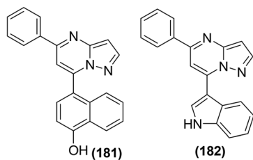
Fig. 58 Chemical structures of selected 7-(hetero)aryl-substituted pyrazolo[1,5-a]pyrimidines (181 and 182).
