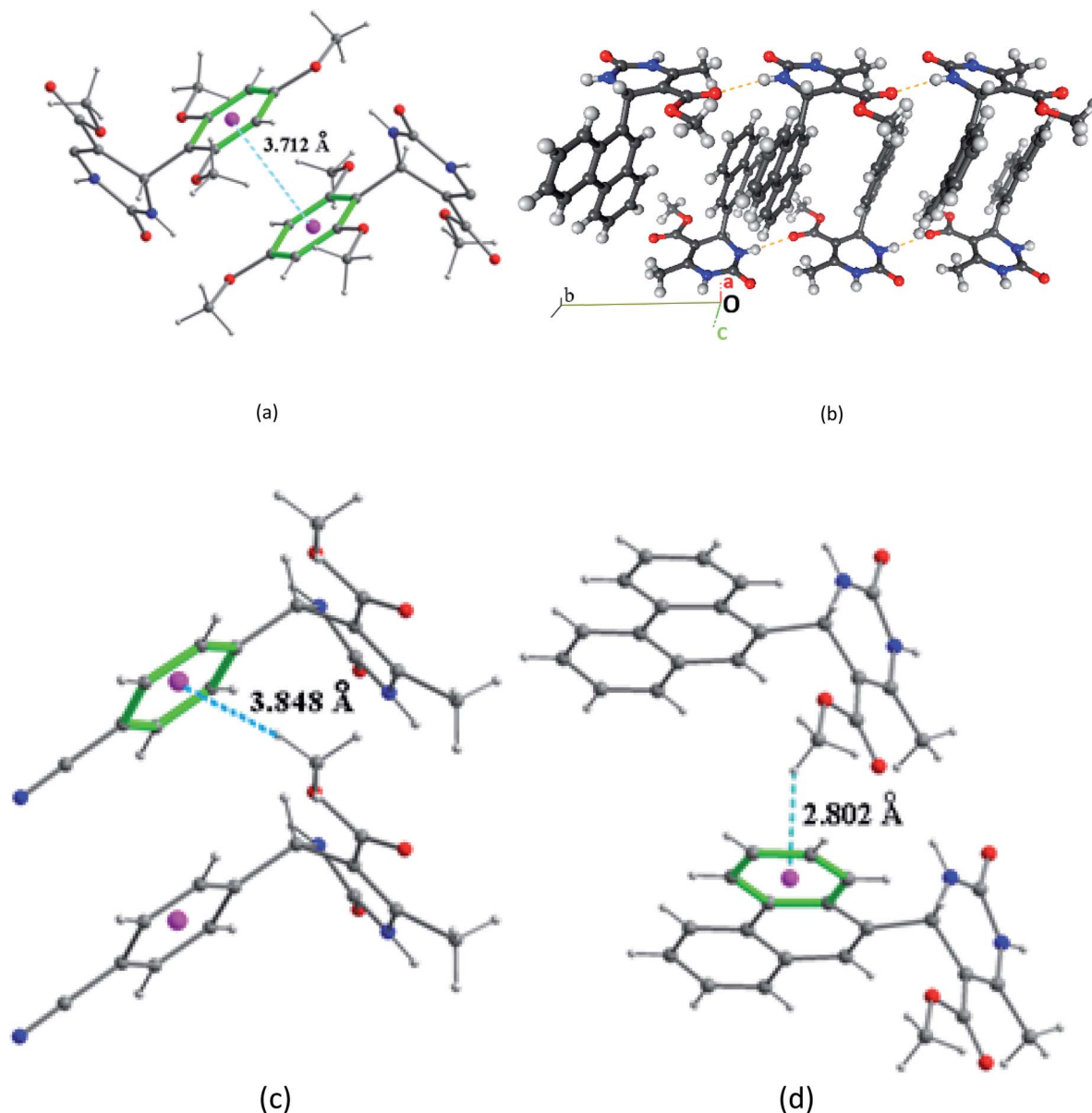
Fig. 7 Intermolecular aromatic stacking interactions between the neighboring aromatic rings: (a) in compound 2, (b) in compound 7 (autotereogram with horizontal translation along b ). Intermolecular C–H... \pi interactions: (c) in compound 3, (d) compound 7.
