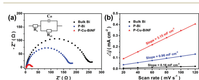
Fig. 5 (a) Electrochemical impedance plots and (b) capacitive \Delta j ( =j_a - j_c ) against scan rate for P-Cu-BiNF, P-Bi and bulk Bi.
