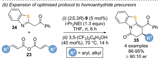
Scheme 10 Selective Michael–lactamization or Michael–lactonization using aryl esters.
