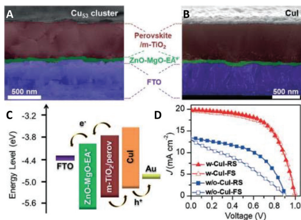
Fig. 38 Device structure and cross-sectional SEM image of (A) Cu 53 and (B) CuI on perovskite films. (C) Energy-level diagram of CuI-based perovskite solar cell (PSC). (D) Best J - V curves of devices with CuI (w-CuI) and without CuI (w/o-CuI). FS = forward scan, RS = reverse scan. Adapted with permission from ref. 194. Copyright 2019 Wiley-VCH Verlag GmbH & Co. KGaA, Weinheim.
