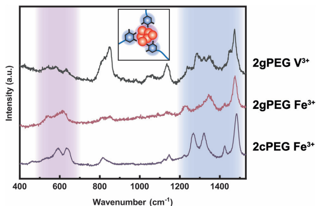
Fig. 5 Raman characterization of 2gPEG hydrogels. Resonance Raman spectra of 2gPEG crosslinked with V^{3+} and Fe^{3+} , and 2cPEG crosslinked with Fe^{3+} . The peaks between 500 and 680\text{ cm}^{-1} are attributed to the catechol- Fe^{3+} coordination or pyrogallol- Fe^{3+} coordination, while the peaks between 1230 and 1500\text{ cm}^{-1} are due to the carbon ring vibration.
