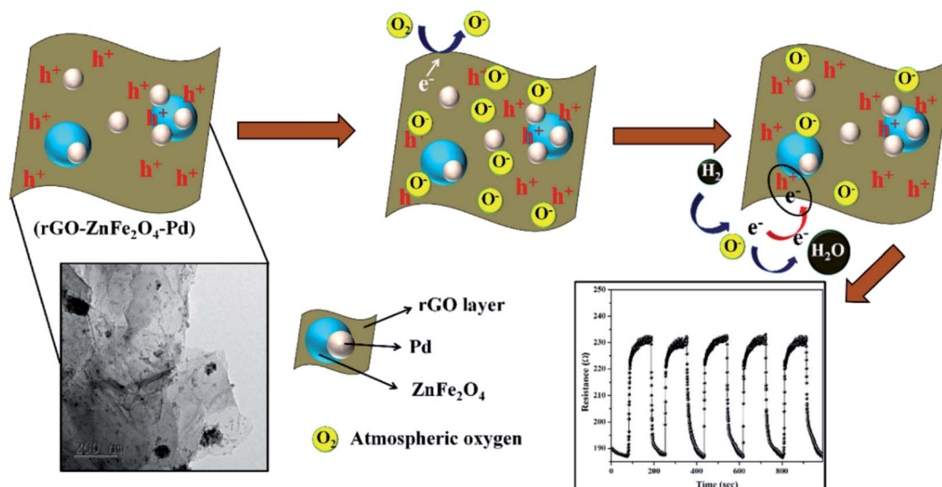
Fig. 14 Plausible sensing mechanism of ZnFe 2 O 4 -Pd decorated rGO towards H 2 gas 190 (reprinted from ref. 190. Copyright (2020), with permission from Elsevier).
