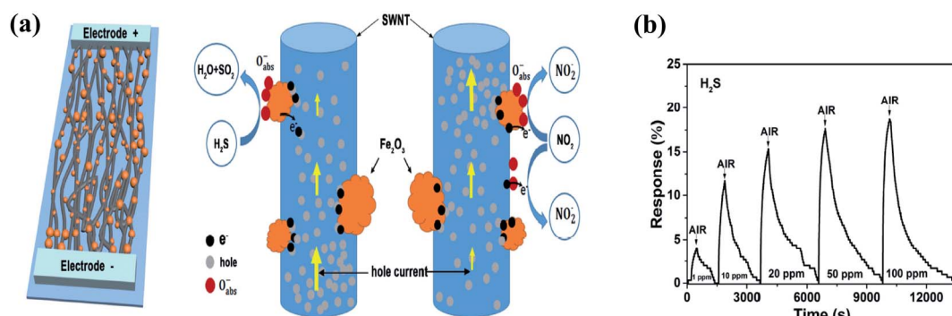
Fig. 15 (a) Schematic of the gas sensor based on SWNT-Fe 2 O 3 composite film and schematic explaining the H 2 S sensing mechanism. (b) Response ( \Delta R/R_a ) and recovery curves of sensor upon exposure to H 2 S (1, 10, 20, 50, and 100 ppm) with complete recovery 107 (reprinted from ref. 107. Copyright (2017), with permission from Elsevier).
