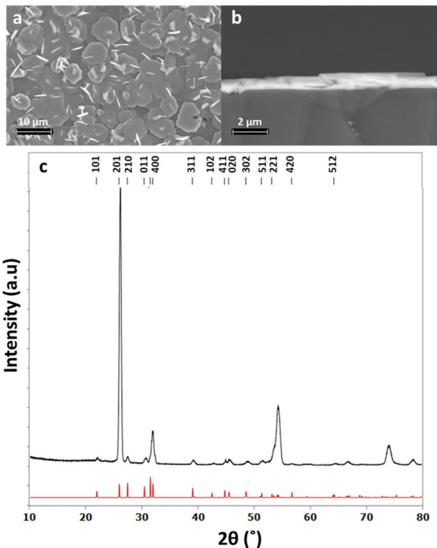
Fig. 4 Top down SEM image (a), cross sectional SEM image (b) and grazing incidence XRD pattern (c) for SnS thin film obtained by low pressure CVD using [\text{Sn}^n\text{Bu}(\text{S}^n\text{Bu})_2] (red = XRD pattern for bulk \text{SnS}^{48} ) with a thickness of around 700 nm.
