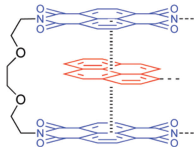
Fig. 9 Structure of the electronically complementary \pi - \pi stacking interaction between a bis(diimide) chain fold in polyimide [reproduced from ref. 11 with permission from the ACS].
