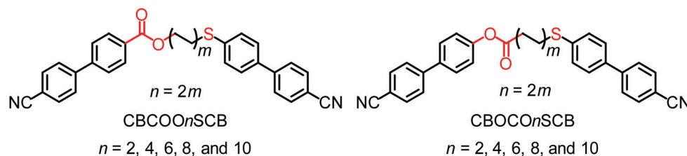
Fig. 1 Molecular structures of CBCOO_nSCB ( n = 2, 4, 6, 8, \text{ and } 10 ) and CBOCO_nSCB ( n = 2, 4, 6, 8, \text{ and } 10 ), where n = 2m .
