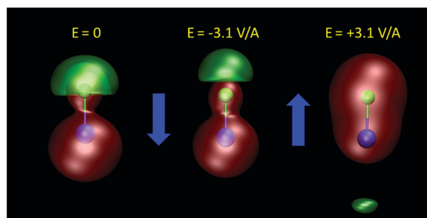
Fig. 9 The QM response of a NaCl molecule in an applied electric field E = \pm 3.1 V Å -1 (field direction indicated by blue arrows). The resulting potential isosurfaces (red = positive, green = negative) and total dipole moments are: V = \pm 2 V and \mu = 9 D (left), V = \pm 3.5 V and \mu = 14.3 D (middle), V = \pm 3.5 V and \mu = -24.7 D (right). QM level: B3LYP/aug-cc-pvdz.
