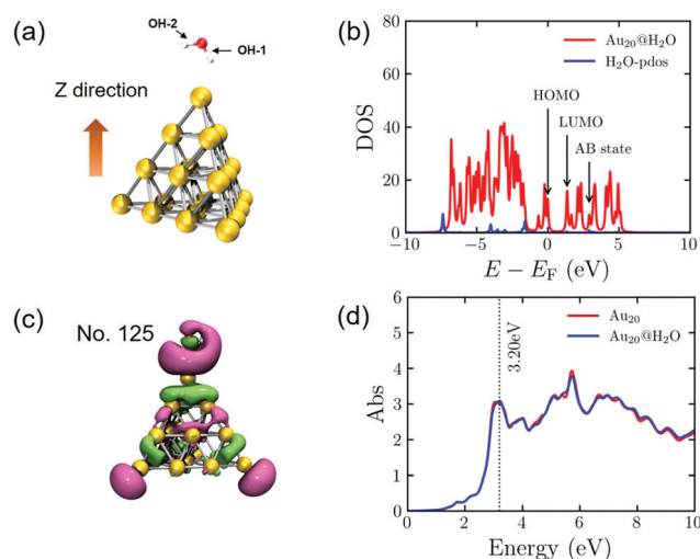
Fig. 1 (a) The optimized \text{Au}_{20}@H_2O geometry. (b) The DOS of \text{Au}_{20}@H_2O (Fermi-level is set to zero) and PDOS of the H_2O molecule (in blue), where we mark the HOMO (No. 114) and LUMO (No. 115, 1.35 eV) of the hybrid system, and the orbital with antibonding (AB) characteristics, namely, AB state (No. 125, 2.95 eV). (c) The MO of No. 125. (d) The absorption spectra of \text{Au}_{20}@H_2O and \text{Au}_{20} .
