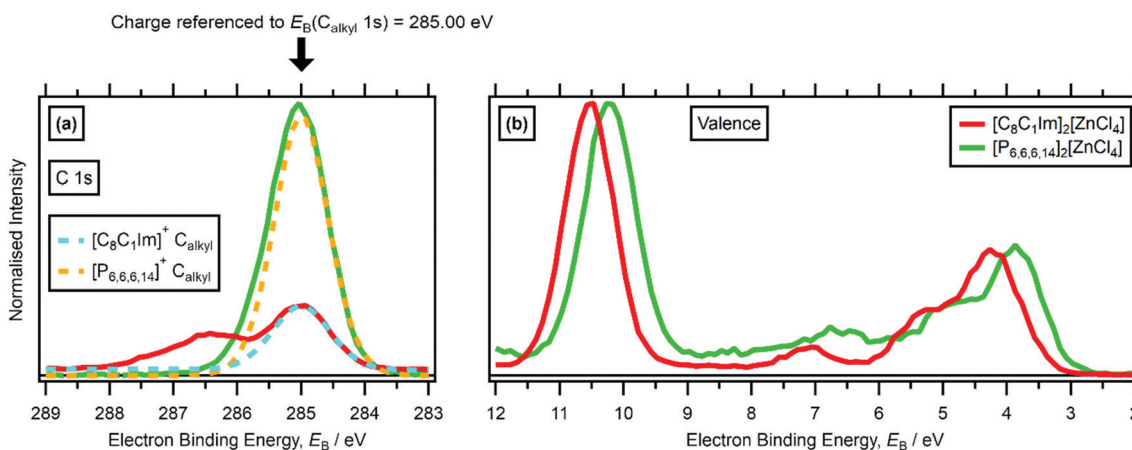
Fig. 5 Non-resonant laboratory XPS at h\nu = 1486.6 eV for [C_8C_1\text{Im}]_2[\text{ZnCl}_4] and [P_{6,6,6,14}]_2[\text{ZnCl}_4] : (a) C 1s, (b) valence. XP spectra were charge referenced to E_B(C_{\text{alkyl}} 1s) = 285.00 eV ( i.e. using method 1 outlined in Section 2.5).
