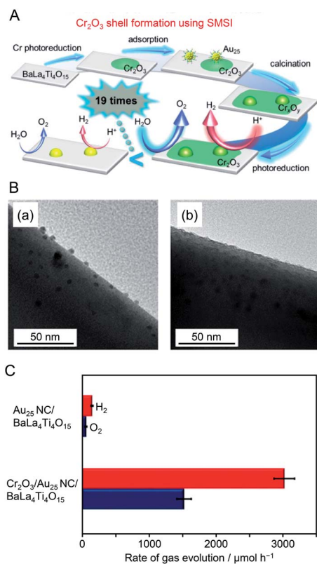
Fig. 16 (A) Schematic of the preparation of \text{Cr}_2\text{O}_3/\text{Au}_{25} NC/ \text{BaLa}_4\text{Ti}_4\text{O}_{15} . (B) TEM images of (a) \text{Au}_{25} NC/ \text{BaLa}_4\text{Ti}_4\text{O}_{15} and (b) \text{Cr}_2\text{O}_3/\text{Au}_{25} NC/ \text{BaLa}_4\text{Ti}_4\text{O}_{15} after UV irradiation for 10 h. (C) Comparison of rates of \text{H}_2 and \text{O}_2 evolution by photocatalytic water splitting over \text{Au}_{25} NC/ \text{BaLa}_4\text{Ti}_4\text{O}_{15} and \text{Cr}_2\text{O}_3/\text{Au}_{25} NC/ \text{BaLa}_4\text{Ti}_4\text{O}_{15} (0.5 wt% Cr). Averages of values obtained from several experiments are shown. Reproduced with permission from ref. 190. Copyright 2018 American Chemical Society.
