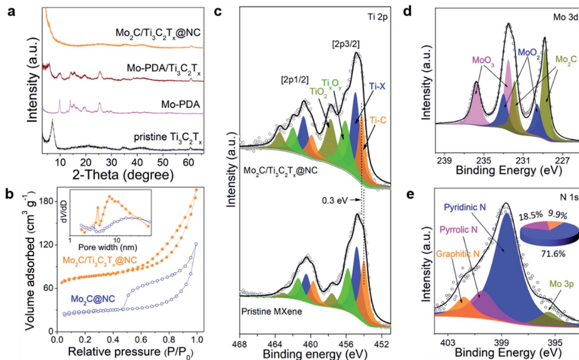
Fig. 3 (a) XRD patterns of pristine \text{Ti}_3\text{C}_2\text{T}_x MXene, Mo-PDA, Mo-PDA/ \text{Ti}_3\text{C}_2\text{T}_x and \text{Mo}_2\text{C}/\text{Ti}_3\text{C}_2\text{T}_x@NC . (b) \text{N}_2 adsorption–desorption isotherms and the corresponding pore size distributions of \text{Mo}_2\text{C}@NC and \text{Mo}_2\text{C}/\text{Ti}_3\text{C}_2\text{T}_x@NC . High-resolution XPS spectra of (c) Ti 2p, (d) Mo 3d and (e) N 1s of \text{Mo}_2\text{C}/\text{Ti}_3\text{C}_2\text{T}_x@NC . The Ti 2p survey of pristine \text{Ti}_3\text{C}_2\text{T}_x MXene is presented in (c) for comparison. The inset in (e) is the calculated contents of pyridinic N, pyrrolic N and graphitic N in \text{Mo}_2\text{C}/\text{Ti}_3\text{C}_2\text{T}_x@NC .
