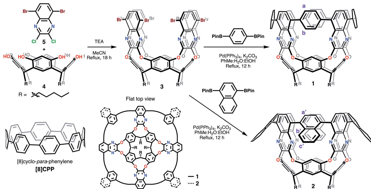
Scheme 1 Synthesis of tubular [n_b, n, m, r] arenes 1 and 2.
