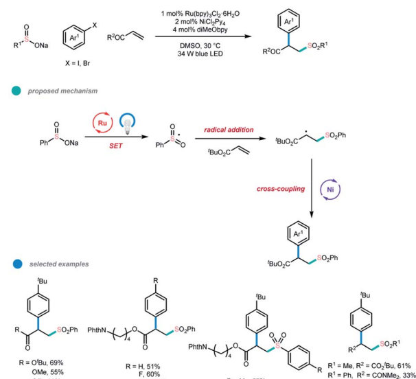
Scheme 16 Three-component arylsulfonylation of alkenes via photoredox and nickel dual catalysis.
