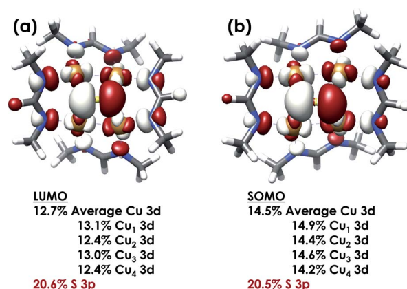
Fig. 5 (a) Restricted Kohn–Sham LUMO for [4\text{Cu}:1\text{S}]^0 and (b) quasi-restricted (QRO) 33 SOMO for [4\text{Cu}:1\text{S}]^{1-} . Both MOs were calculated for truncated models using the B3LYP hybrid density functional with the CP(PPP) basis set on Cu and the scalar-relativistically recontracted ZORA-def2-TZVP(-f) basis set on all other atoms. Orbitals are plotted at an isovalue of 0.03 au.
