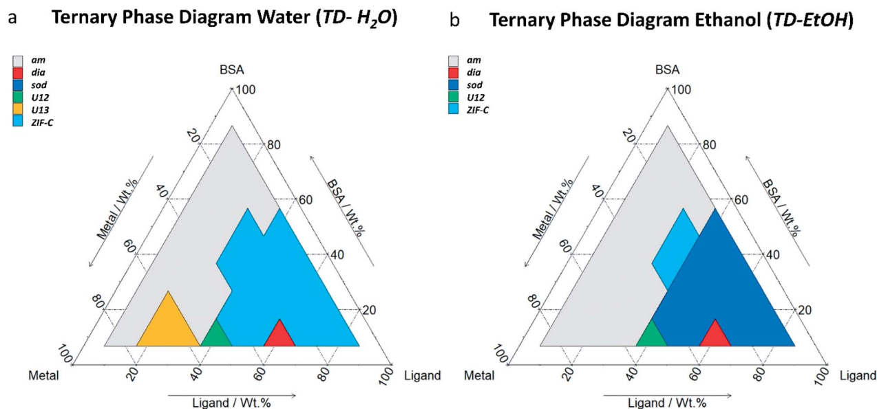
Fig. 1 Ternary diagrams (by weight fraction, see Table S1† for details) of BSA, HmIM (labelled as ligand) and \text{Zn}(\text{OAc})_2 \cdot 2\text{H}_2\text{O} (labelled as metal). TD- \text{H}_2\text{O} (a) represents the main phases (>50 wt, see Table S2† for details) obtained by washing the sample with DI water. TD-EtOH (b) represents the main phases (>50 wt, see Table S3† for details) obtained by washing the sample first with DI water and then with ethanol. The total mass of the reagent was chosen by selecting a value in between those previously reported in the literature (see ESI† for further details). 11,34
