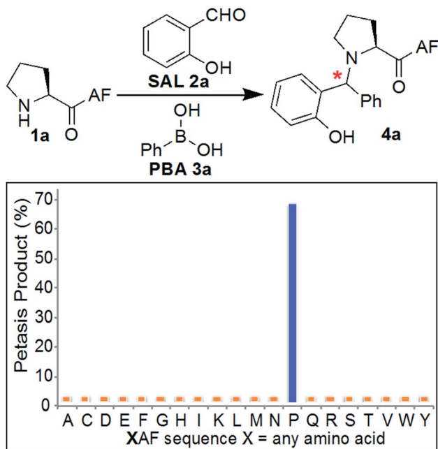
Fig. 3 Chemoselectivity of SASP reaction for N-terminal proline. The reaction showed high selectivity for N-terminal proline as analyzed by LC/MS for a panel of XAF peptides, where X represents a variable amino acid. Reaction conditions: 2 mg XAF (12–17 mM), SAL 2a (3 equiv., 36–51 mM), PBA 3a (4 equiv., 48–68 mM) in buffer (pH 7.3) : DMF (4 : 1) at room temperature for 4–24 h.
