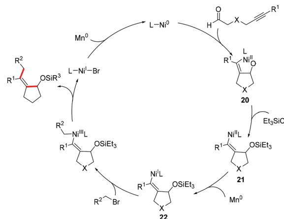
Scheme 17 Ni-Catalyzed reductive coupling of alkynals with alkyl halides.
