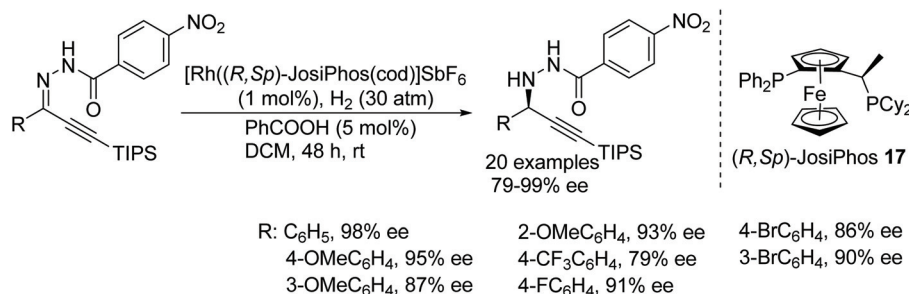
Fig. 24 Chemoselective and enantioselective synthesis of chiral propargyl hydrazines.
